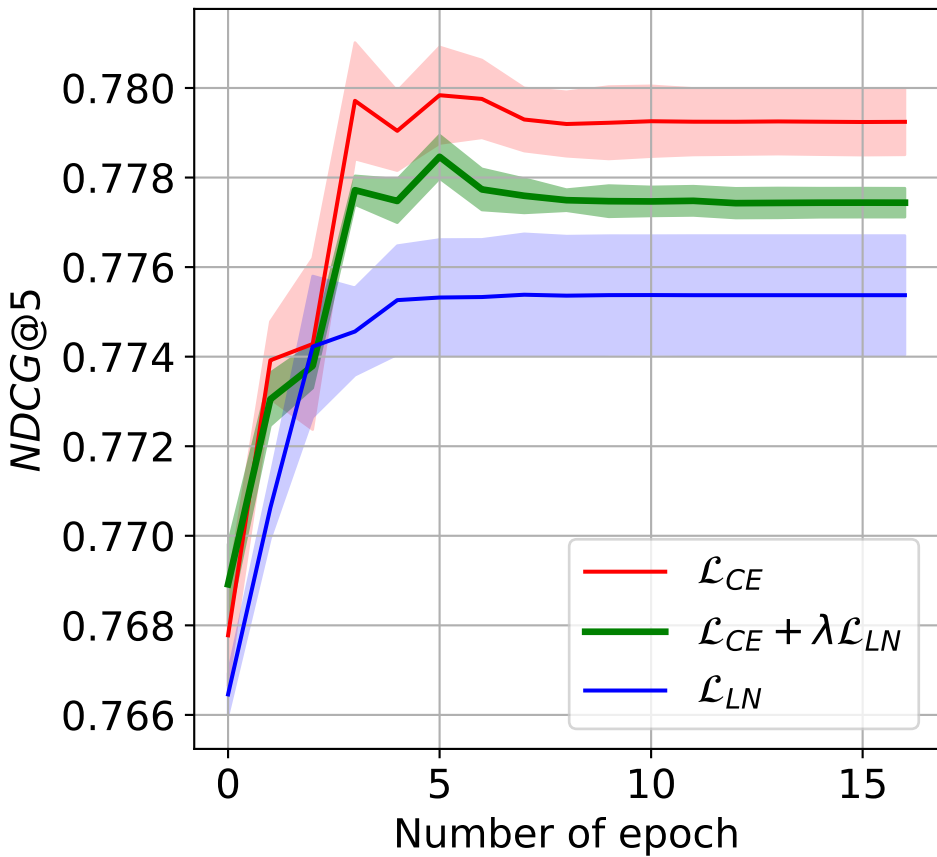
NDCG@5
